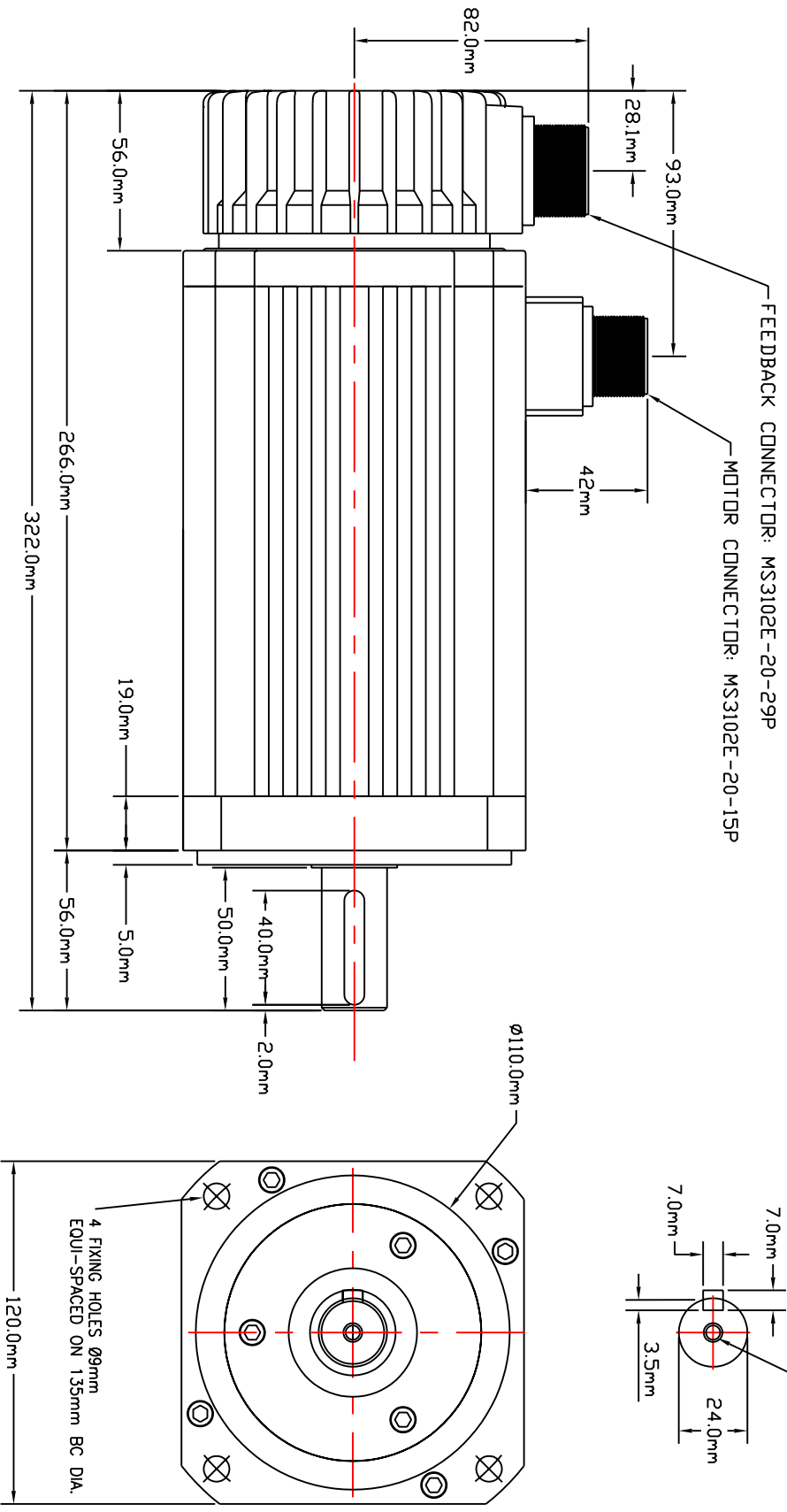
2.2 KILOWATT AC SERVO MOTOR #10688
